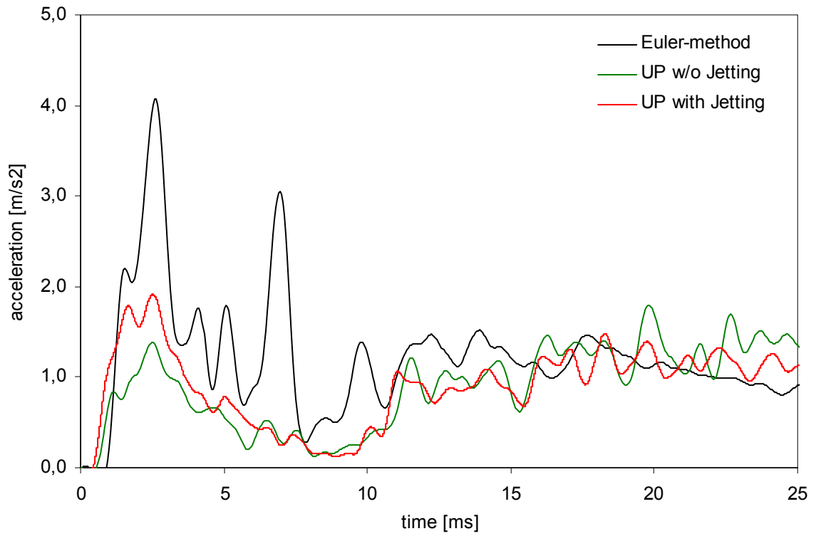
Figure 10: Total acceleration of head with different modeling techniques
