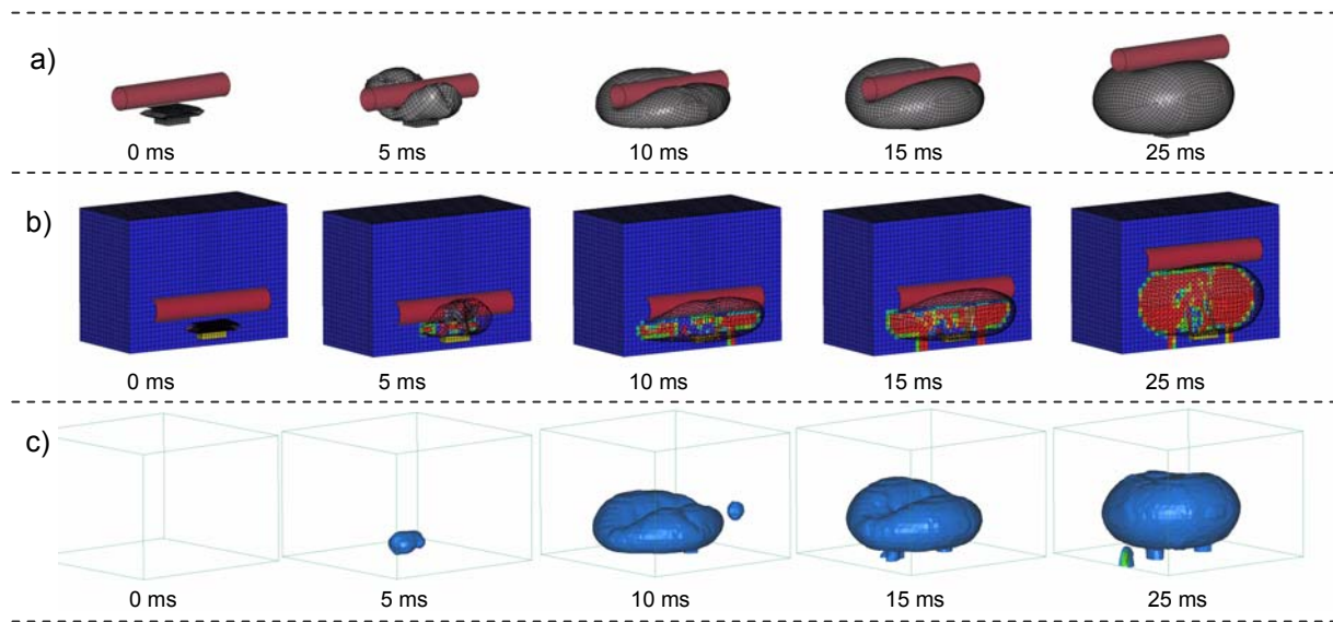
Figure 7: Unfolding of airbag: a) Control-Volume b) Euler-method and c) iso-surface of inflowing gas
