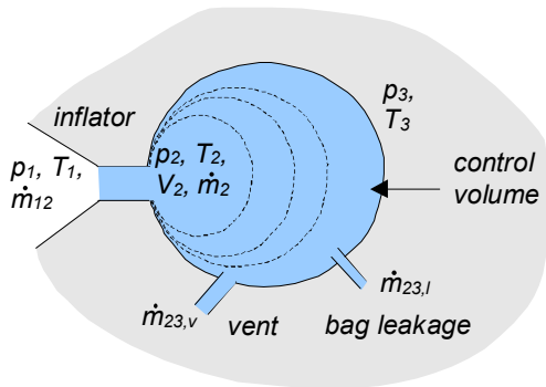
Figure 1: Control-Volume-concept
