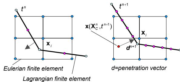
Figure 5: Penalty based coupling concept
