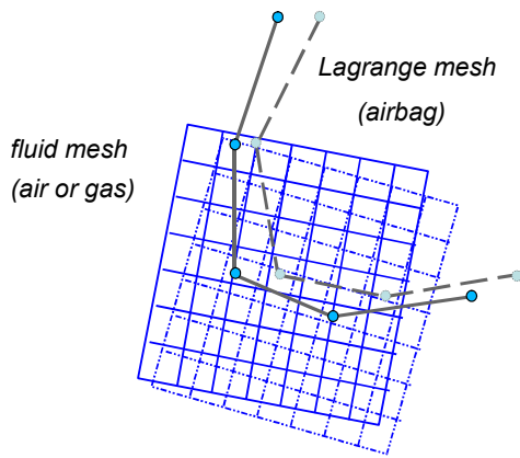
Figure 3: ALE-concept at two adjacent time steps
