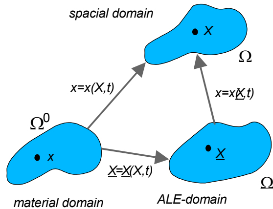
Figure 2: Control-Volume-concept
