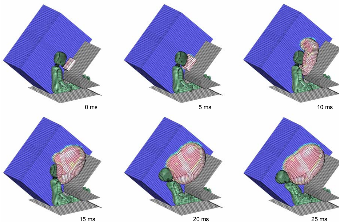
Figure 9: Unfolding of OoP-airbag problem with Euler-method (Euler-mesh cut open)
