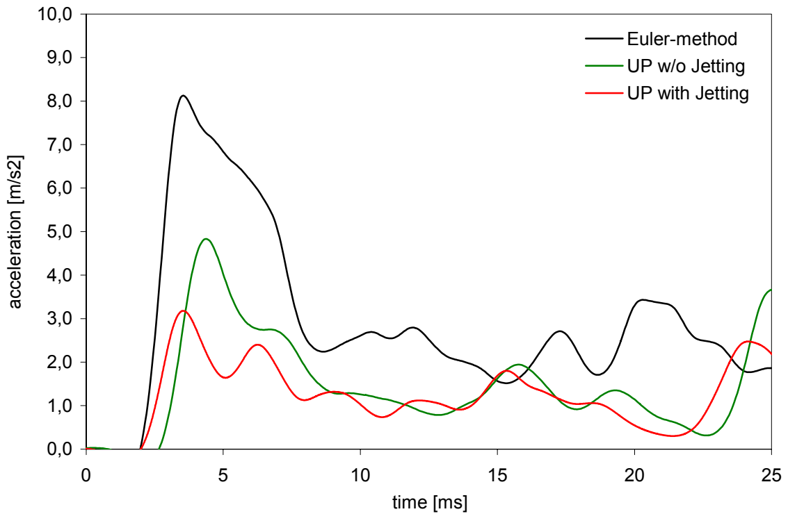
Figure 10: Total acceleration of head with different modeling techniques
