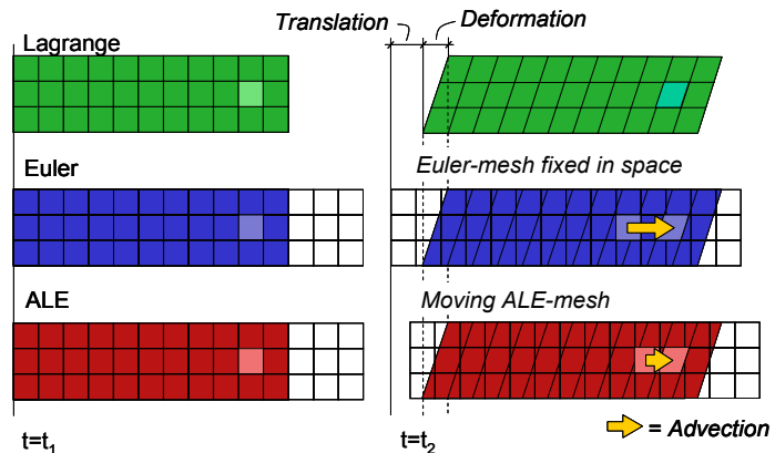
Figure 4: Comparison of Lagrange, Euler and ALE-description
