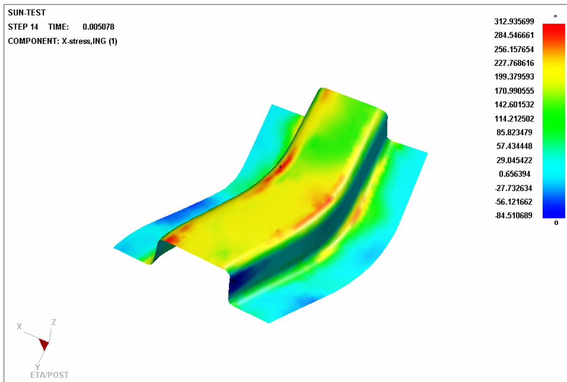
Figure 5.1.9 An Example for PARTIAL MODEL display
