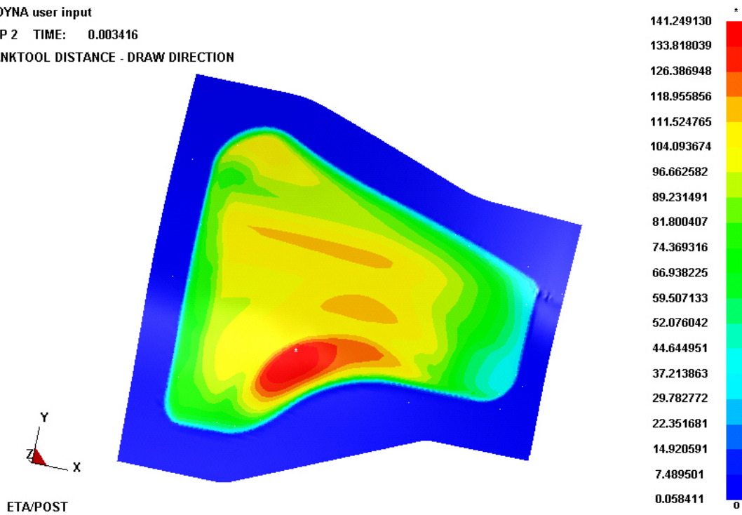
Figure 7.8.3 Blank and Tool Distance
