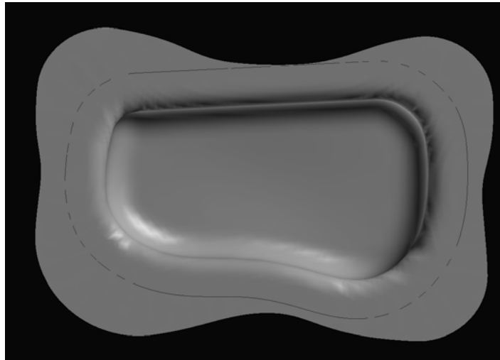
Figure 7.11.2 Trim Line on Final Step of the Deformed Blank
