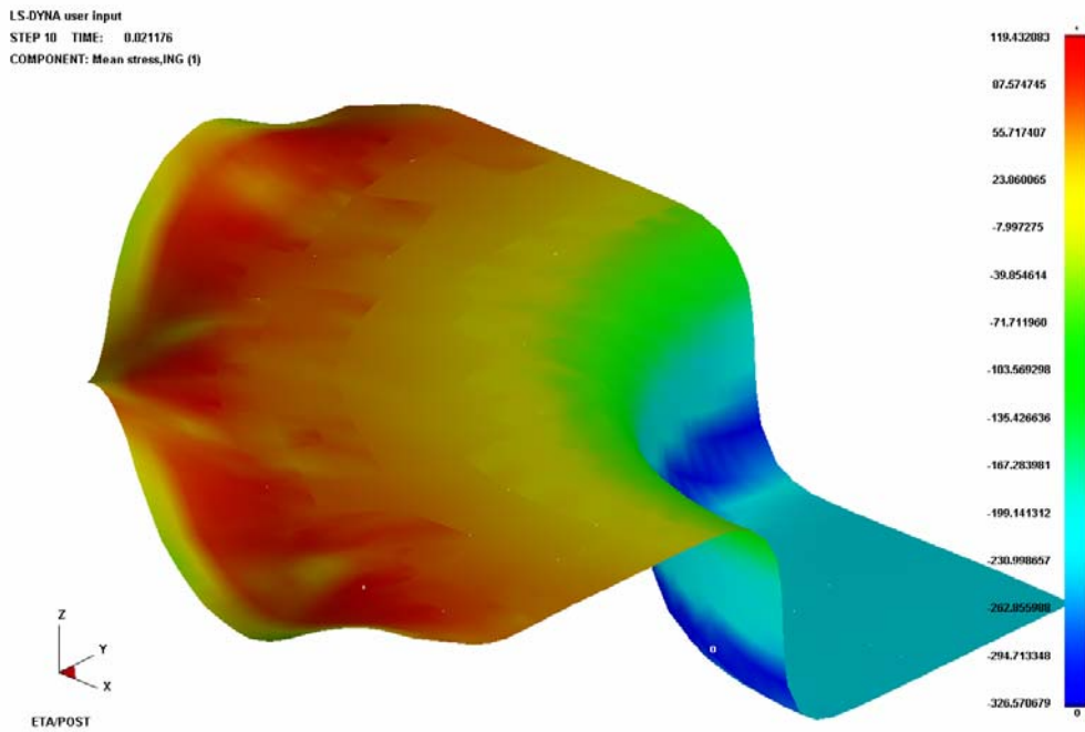
Figure 7.2.3 Contour display on deformed mesh
