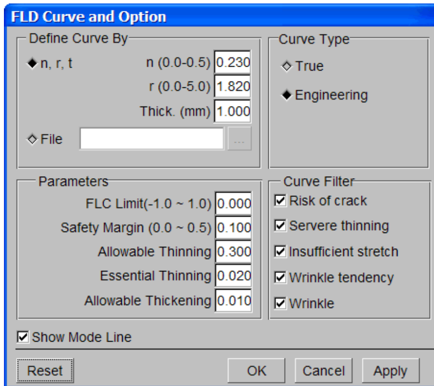
Figure 7.4.2 FLD Curve and Option
