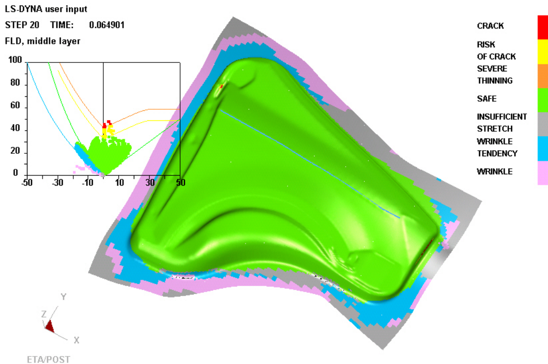
Figure 7.4.3 An Example of FLD evolution
