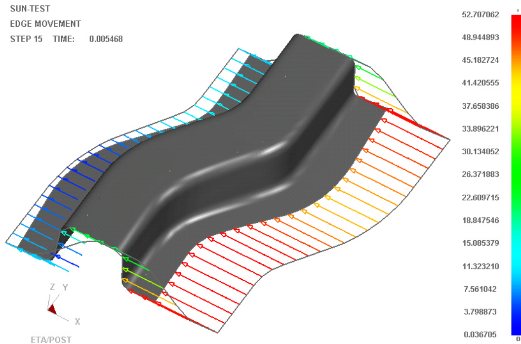
Figure 7.12.2 Edge movement with delta x=20 and reference frame=1.
