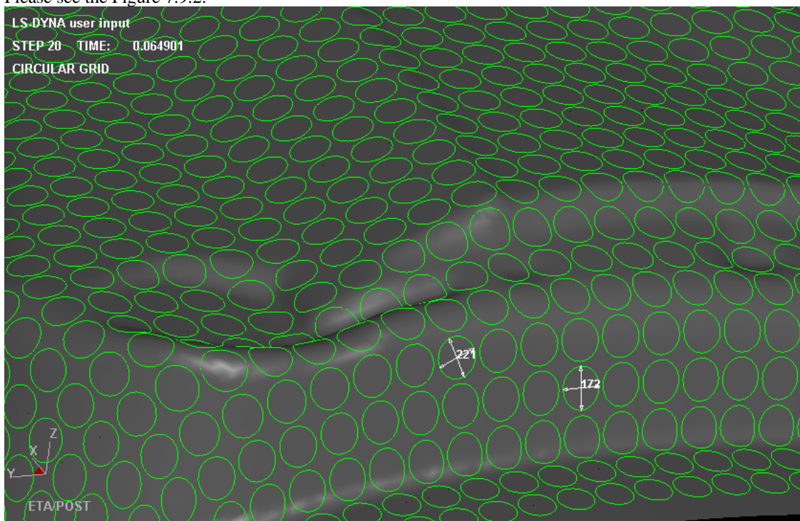
Figure 7.9.2 A sample plot of Circular Grid
