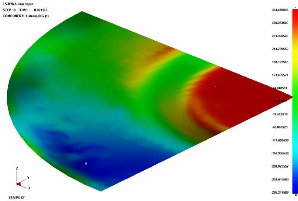
Figure 7.2.2 Contour display on un-deformed mesh
