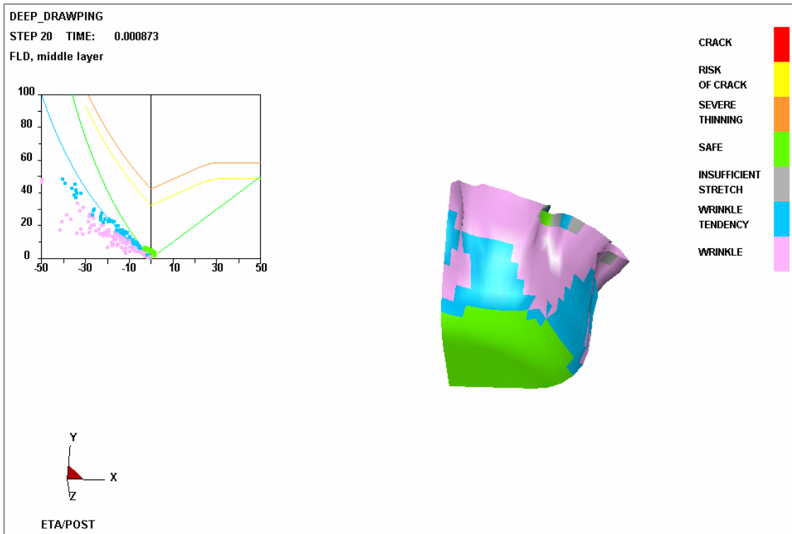
Figure 5.3.2 Example of a quarter model and result
