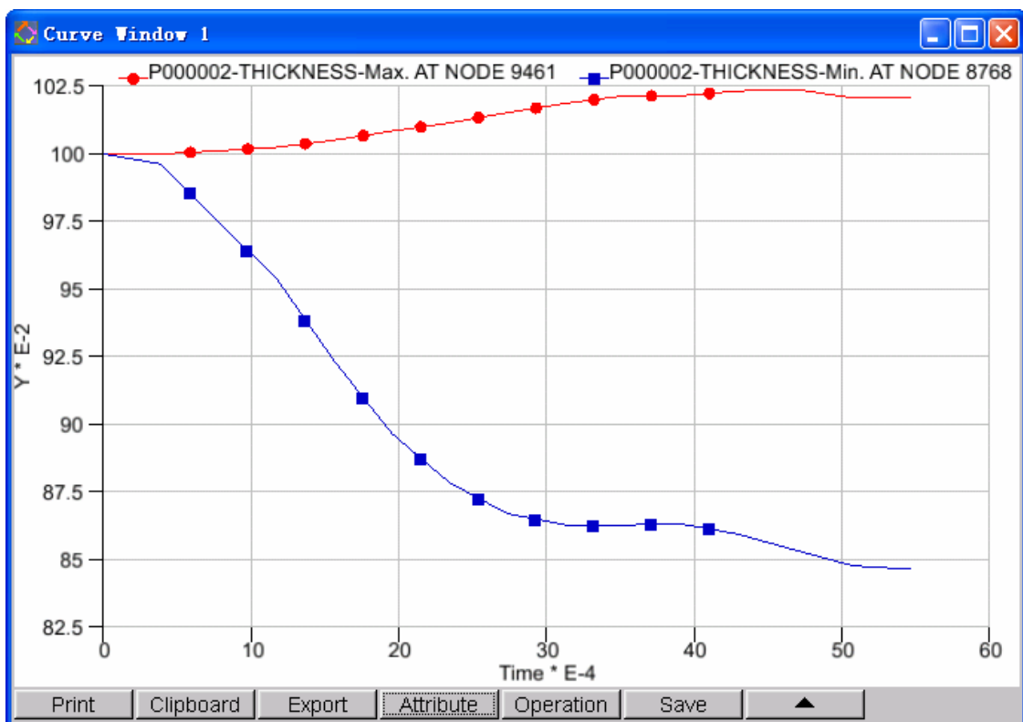
Figure 5.6.2 A typical Part value curve
