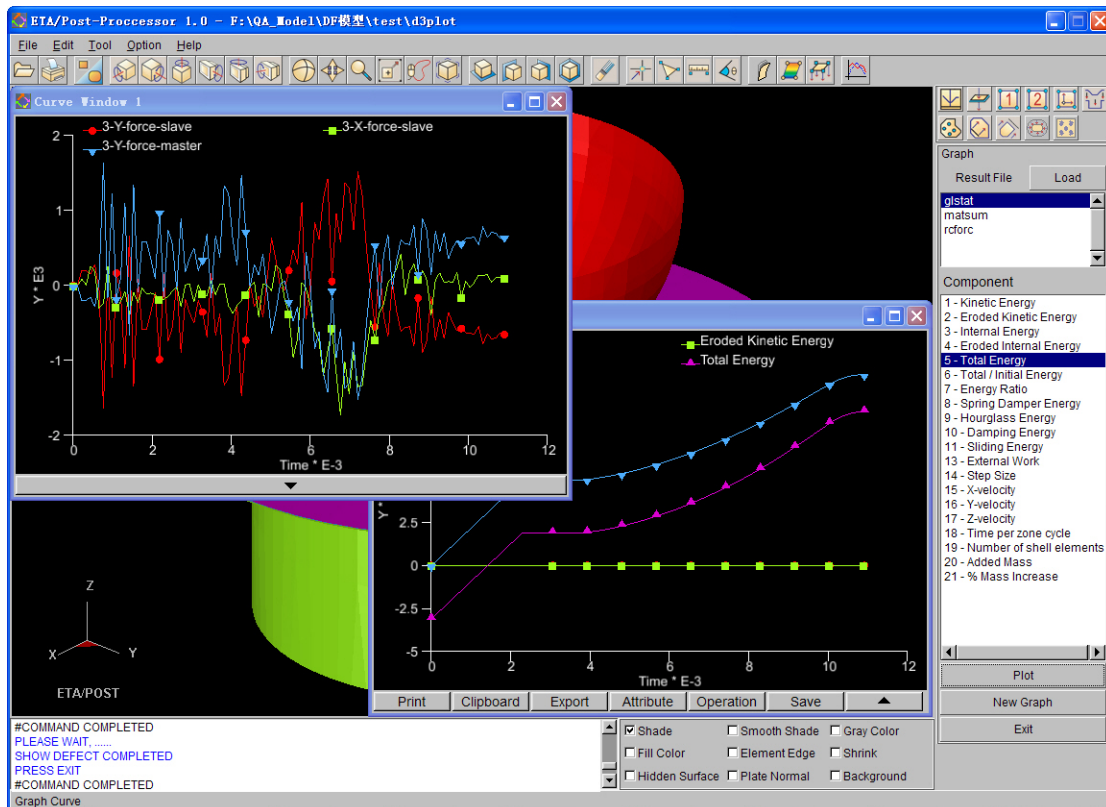
Figure 7.14.4 Graph window in eta-Post window.
