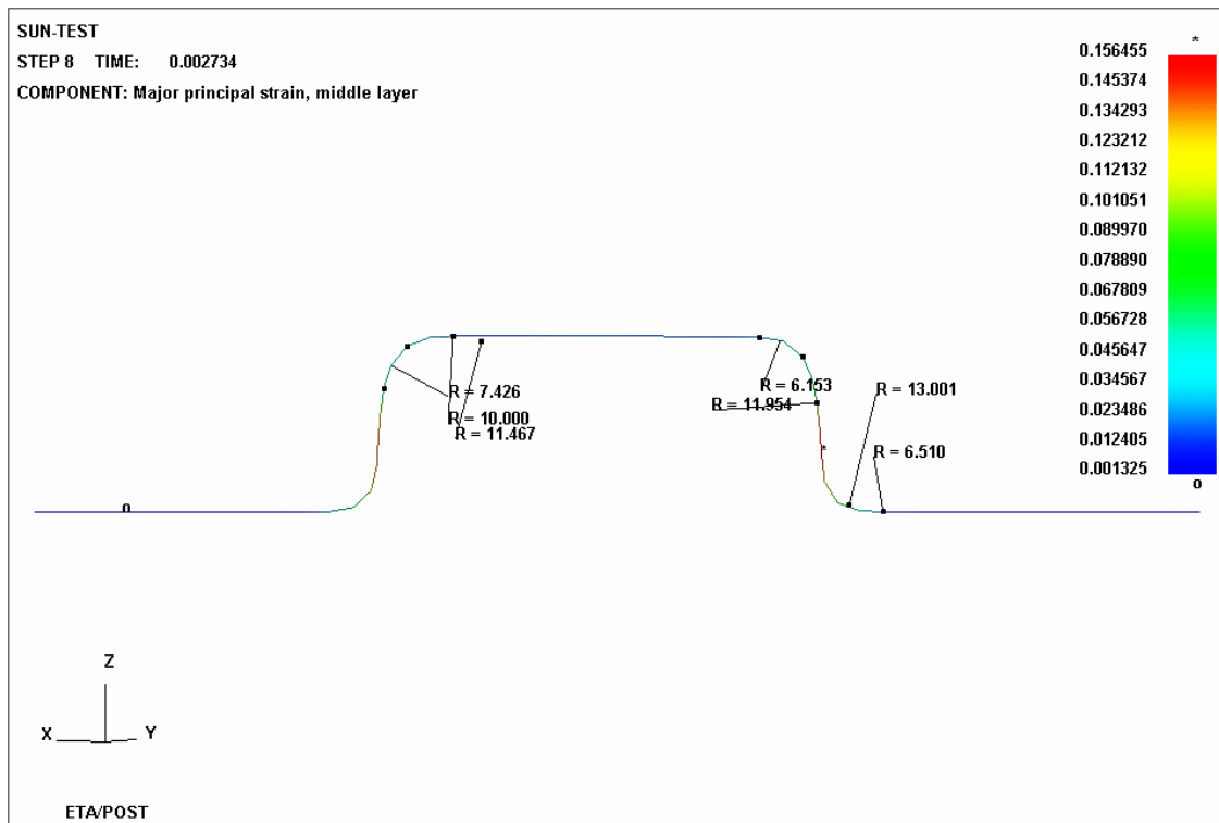
Figure 5.1.5 The result of ARC FIT
